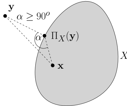
Figure 3.1: Illustration of Fact 3.1
